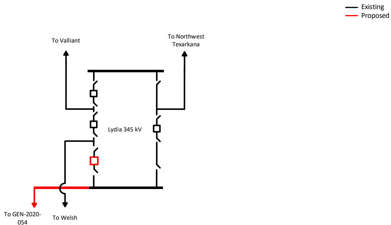
Figure 2: Point of Interconnection Maps
